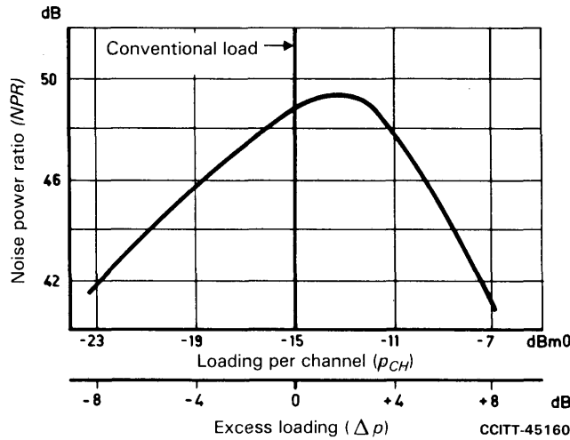
FIGURE A-2/G.228 NPR curve versus channel loading
