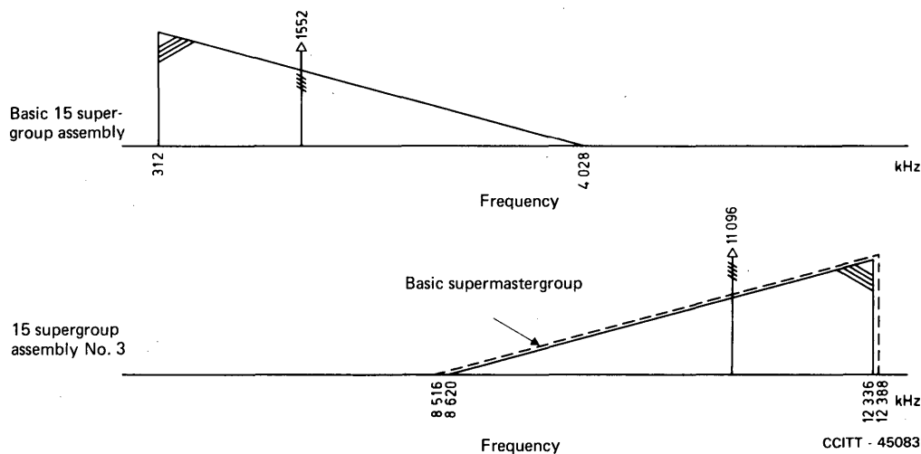
c) Frequency bands occupied by basic 15-super group assembly and by 15-super group assembly No. 3
