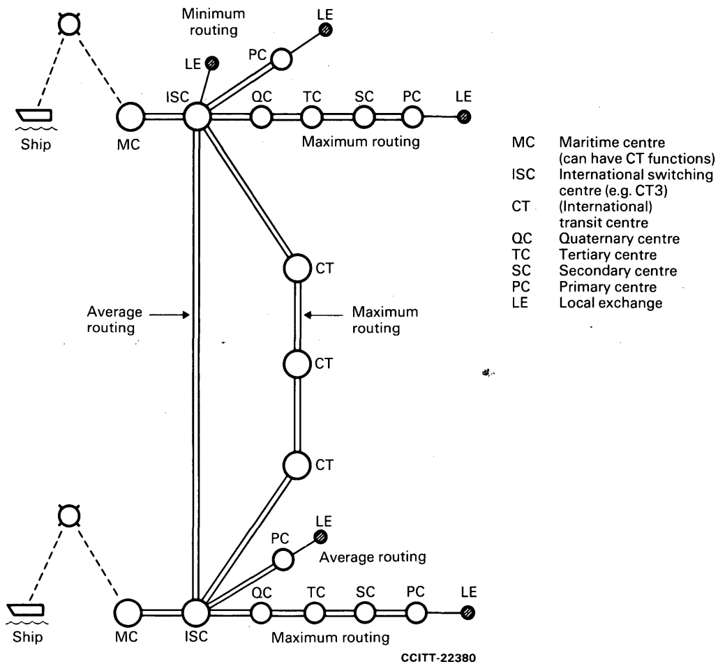
FIGURE 3 Possible routings involving the maritime mobile satellite service (based on Recommendation G.473)
