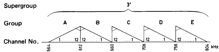
a) Arrangement of groups and channels (supergroup 3' has been shown as an example)
