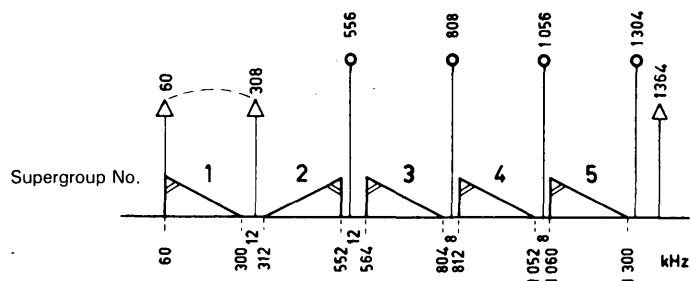
a) Supergroups Nos. 1 to 5 arrangement
