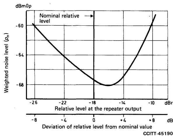
FIGURE A-5/G.228 Weighted noise level in measuring channel versus relative level at repeater output
