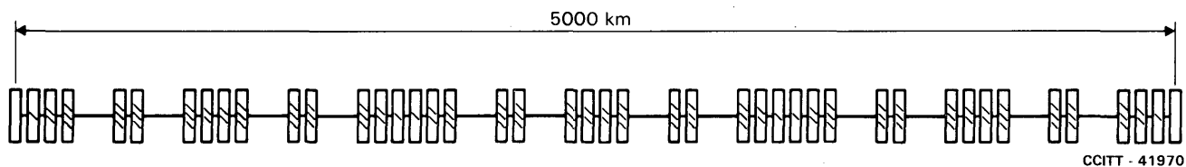
FIGURE 1/G.215 Diagram of a hypothetical reference circuit of 5000 km
