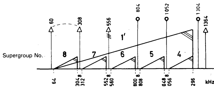
b) Mastergroup arrangement CCITT - 36770
