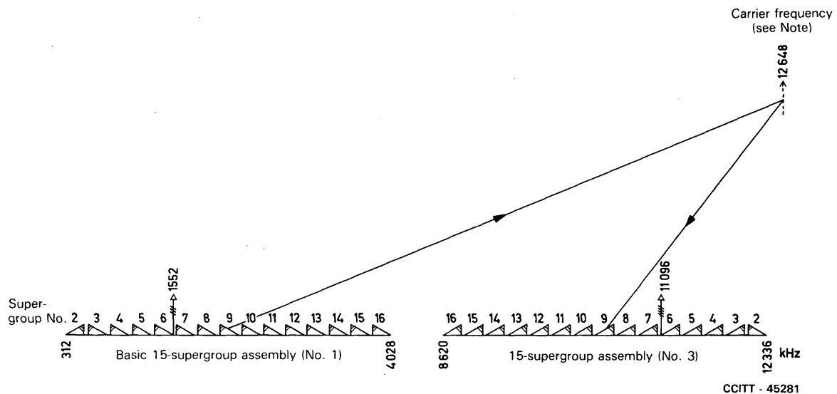
FIGURE 5/G.233 Constitution of 15-supergroup assembly No. 3
