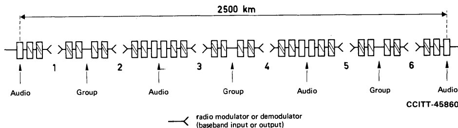
FIGURE 1/G.431 Hypothetical reference circuit for frequency-division multiplex radio-relay systems with a capacity of 12 to 60 telephone channels per radio channel
