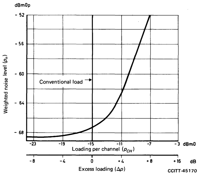
FIGURE A-3/G.228 Weighted noise power level versus system load (relative levels of the system fixed according to plan)
