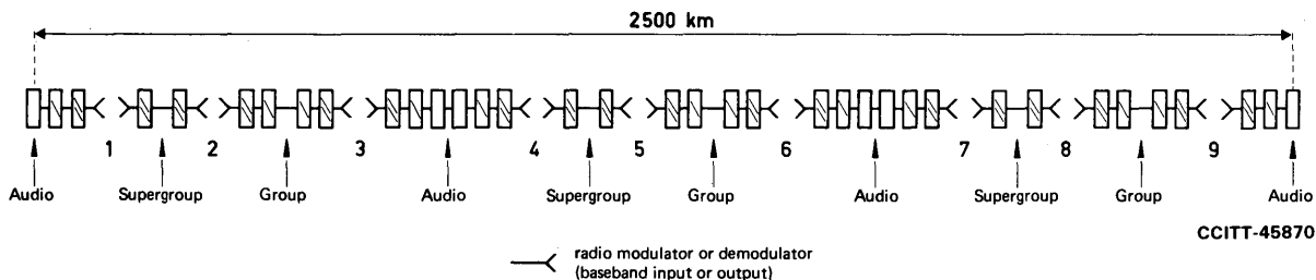
FIGURE 2/G.431 Hypothetical reference circuit for frequency-division multiplex radio-relay systems with more than 60 telephone channels per radio channel
