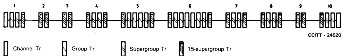
FIGURE 5/G.334 Diagram of a hypothetical reference circuit for 18-MHz systems (Plan 2)
