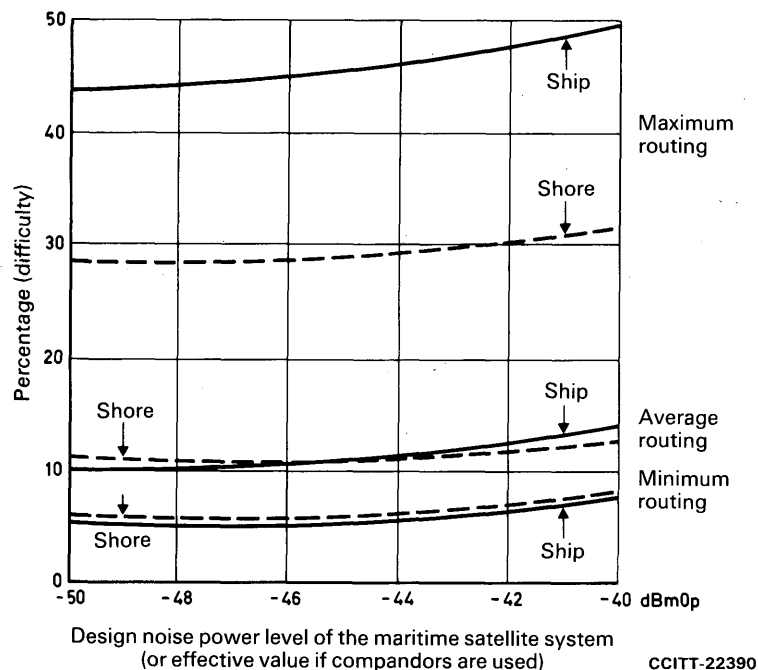
FIGURE 4 Subjective effect of satellite system noise for various routings
