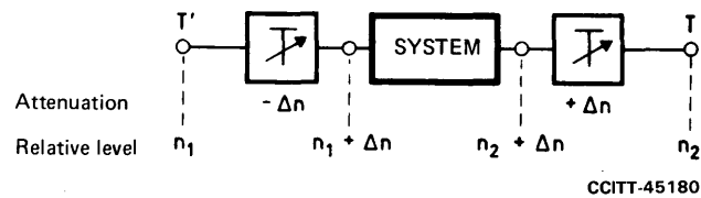
FIGURE A-4/G.228 Variation of the internal relative levels of the system
