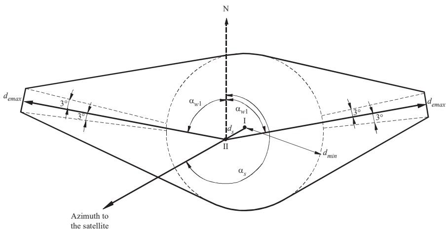
FIGURE 9 Example of the bidirectionnal rain scatter area (Not to scale)
