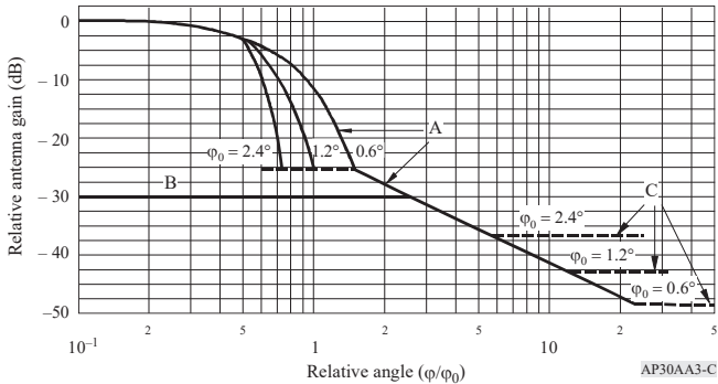
FIGURE C Reference patterns for co-polar and cross-polar components for satellite receiving antennas with fast roll-off in the main beam for Regions 1 and 3
