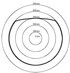
FIGURE 1 Examples of coordination contours for each of the sharing scenarios listed in § 1.4
