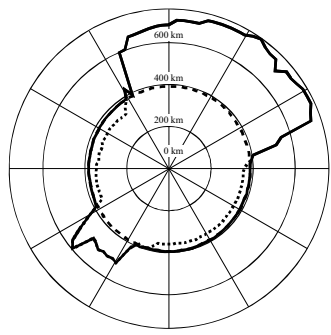
FIGURE 1 Examples of coordination contours for each of the sharing scenarios listed in § 1.4
